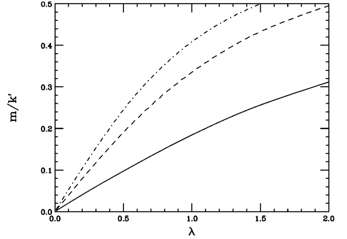
FIG. 10. The same as Fig. 9 but for 0 \leq \lambda \leq 2 and 0 \leq m/k' \leq 0.5 .
