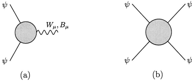
FIG. 7. Diagrams giving flavor nonuniversal gauge interactions (a) and four-fermion operators (b). The gray disks represent the dynamics of the G sector.
