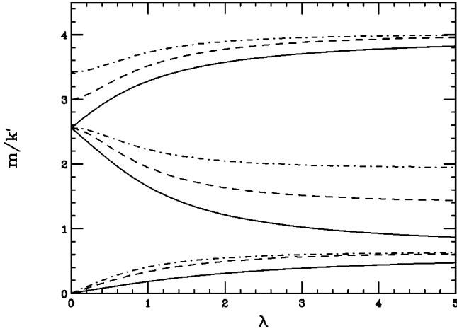
FIG. 9. The spectra for the top KK tower. The horizontal axis is \lambda = y_u H , and the vertical axis is the masses in units of k' . The solid, dashed and dot-dashed lines are for (c_L, c_R) = (0.4, 0.4) , (0.4, 0.1) and (0.4, -0.2) , respectively.
