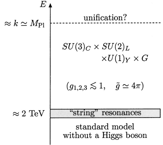
FIG. 11. The overall picture of the theory. Here g_{1,2,3} represents the gauge couplings of SU(3)_C \times SU(2)_L \times U(1)_Y , while \tilde{g} represents that of G .
