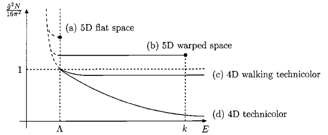
FIG. 1. Schematic description for the evolution of the coupling parameter \kappa \equiv \tilde{g}^2 N / 16\pi^2 in various theories of dynamical electroweak symmetry breaking. The behaviors of (a), (b), (c), and (d) represent those of 5D flat space, 5D warped space, walking technicolor, and technicolor theories, respectively.
