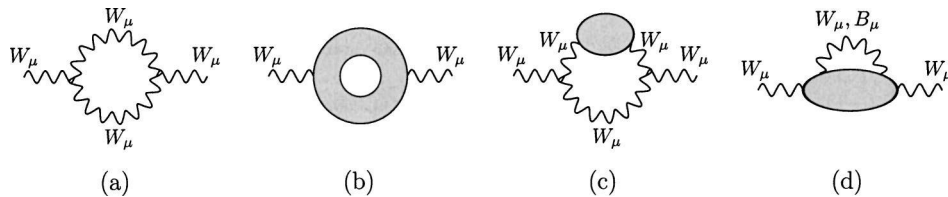
FIG. 5. The diagrams with an elementary loop (a), with the G effect at the next-to-leading order in 1/N (b), and with an additional loop of elementary fields on top of the leading G effect (c), (d). For (a) and (c), similar diagrams using gauge 4-point vertices exist. For (b) and (d), there are also similar diagrams with B_\mu on some of external lines.
