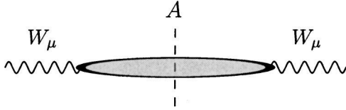
FIG. 4. The diagram representing the mixing between the elementary W boson and the composite W states arising from the dynamics of G . Cutting the diagrams at A gives the states which have the same quantum numbers and spin as W . Similar diagrams also exist for W_\mu replaced by the gauge boson of U(1)_Y , B_\mu .
