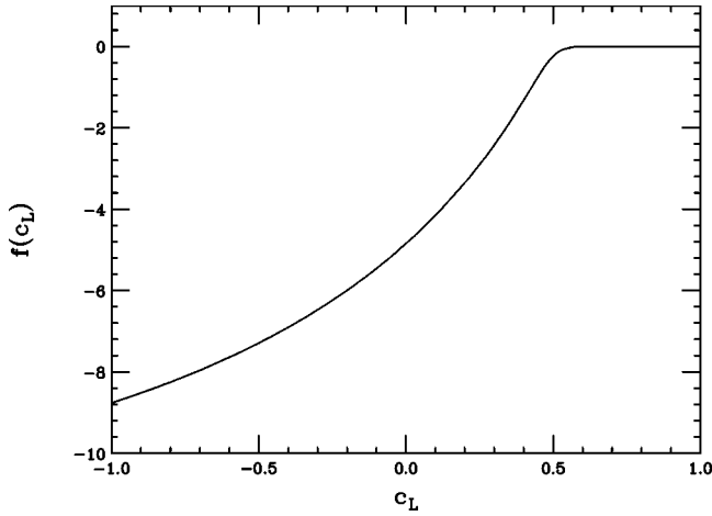
FIG. 8. The function f defined in Eq. (26), which determines the deviation of g_L^b from its standard model value.
