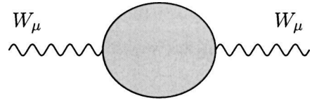
FIG. 2. The diagram contributing to the W boson propagators. Similar diagrams exist with one or two external W_\mu 's replaced by B_\mu .
